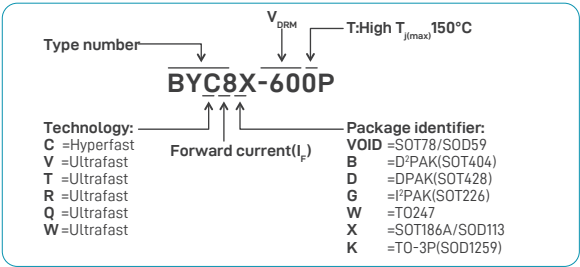
Power Diode part numbering
